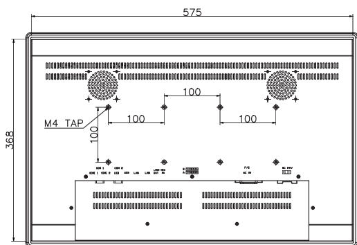
REAR VIEW
